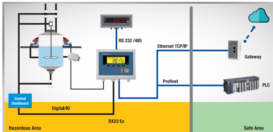
Process control of the vessel in the hazardous area
